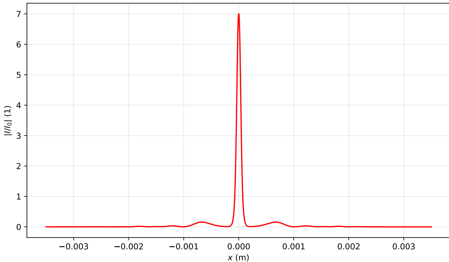
Intensity profile I(x, y = 0, z = 0.637)/I_0 , P_{in}=9.0P_{cr} , artificial time
